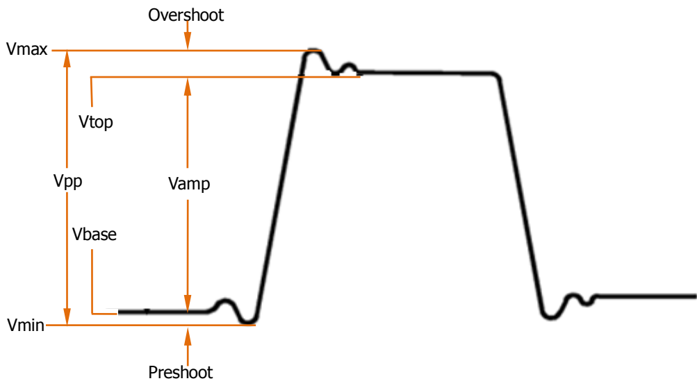
Figure 2-112 Voltage parameters
